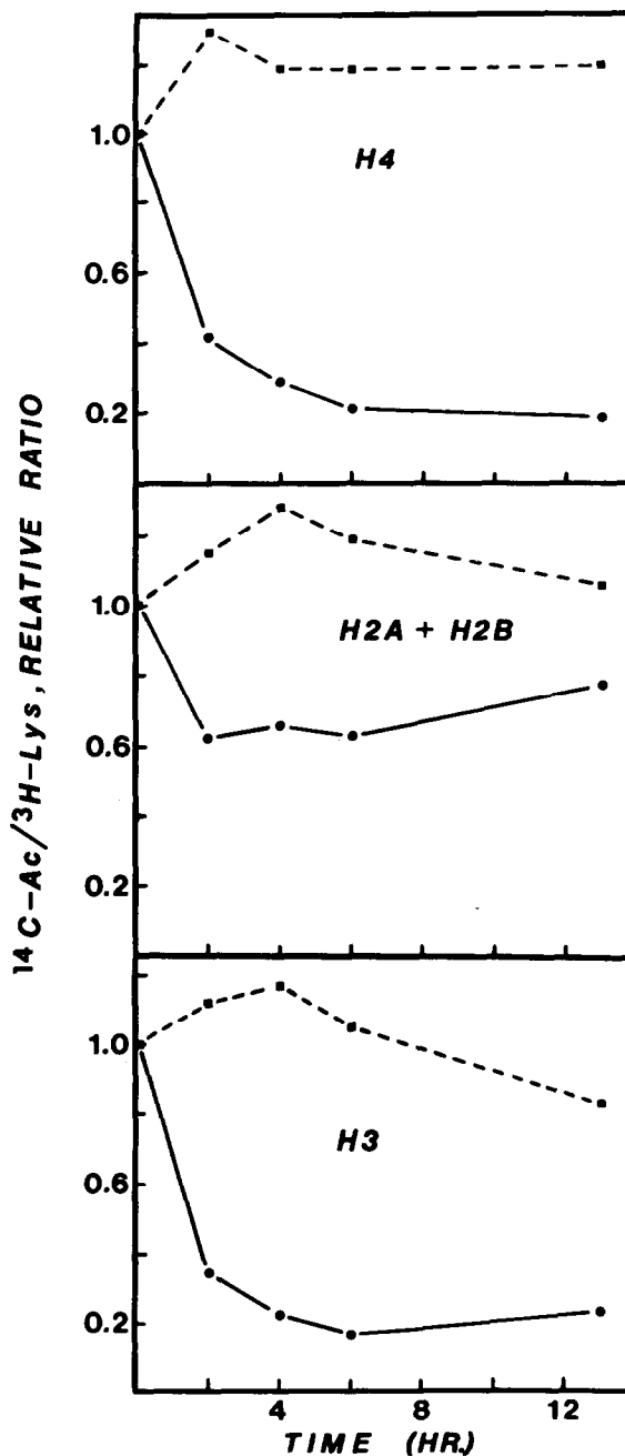
Fig. 1. Pulse labelling of Friend Cells with [ ^{14}\text{C} ]acetate and [ ^3\text{H} ]lysine. Equal numbers of control (C) or butyrate-induced (BA) Friend cells were labelled for 2 h in medium containing [ ^{14}\text{C} ]acetate (150 \mu\text{Ci/ml} ) and [ ^3\text{H} ]lysine (150 \mu\text{Ci/ml} ) at 37^\circ\text{C} . The cells were collected by centrifugation and resuspended in isotope-free medium containing unlabelled acetate (0.1 mM) and lysine (0.5 mM). The cells were then incubated at 37^\circ\text{C} , and aliquots taken at 0, 2 h, 4 h, 6 h and 13 h. For the butyrate-induced cells, 5 mM butyrate was present during both the labelling and chase periods. Chromatin was prepared from each sample, and acid-soluble proteins were extracted and analyzed as in [4].
